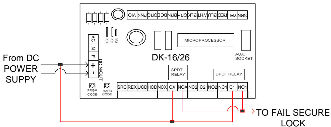
Wiring a DK-16 or DK-26 for HARD CODE Openings & Closings (with a Fail Secure Lock)
